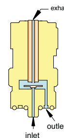
3-Way N.C. Manifold Mount
