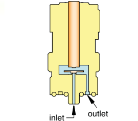
2-Way N.C. Manifold Mount
