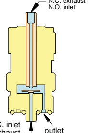
3-Way Manifold Mount
