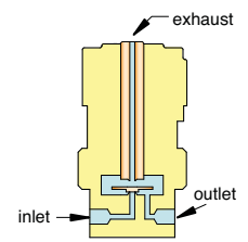
3-Way N.C. In-Line Mount
